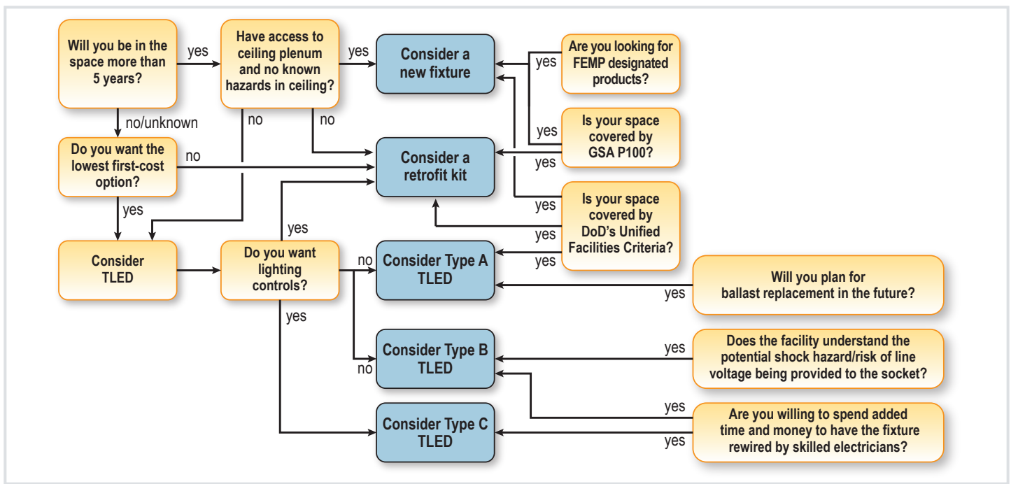
Figure 1. Determining the best LED troffer retrofit option for your facility
